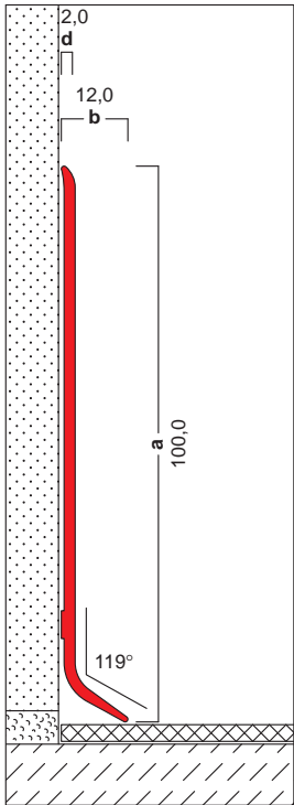
XL 100x12 100,0 x 12,0 mm
